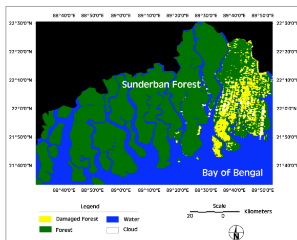
Figure. Damage map of Sunderban caused by Cyclone Sidr 2007. The map was prepared from the Terra MODIS satellite imagery of 18 November 2007 just after the cyclone hit (15 November).
