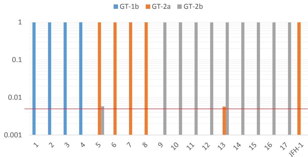
Figure 1. HCV genotypes (GTs) by deep sequencing of HCV NS4 regions. For each sample, only populations that exist at a frequency of >0.005 (red line) were shown by log-scale. No. 5 with the main genotype 2a had minor populations assigned to the different genotype 2b. No. 13 with genotype 2b had minor populations assigned to the different genotype 2a.
